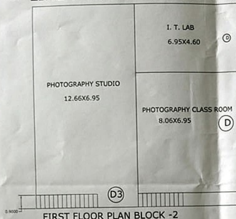
FIRST FLOOR PLAN BLOCK -2
