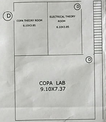
FIRST FLOOR PLAN BLOCK -1
